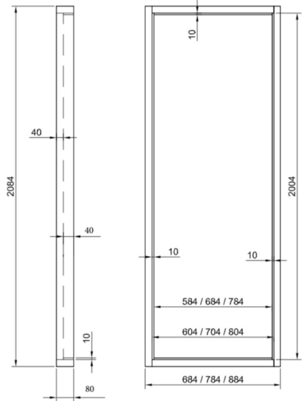
Frame dimensions
